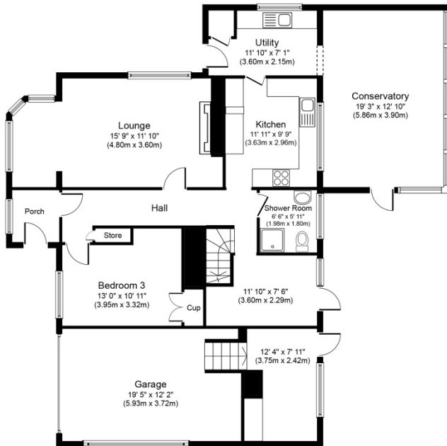
Ground Floor Approximate Floor Area 1,528 sq. ft. (142.0 sq. m.)
