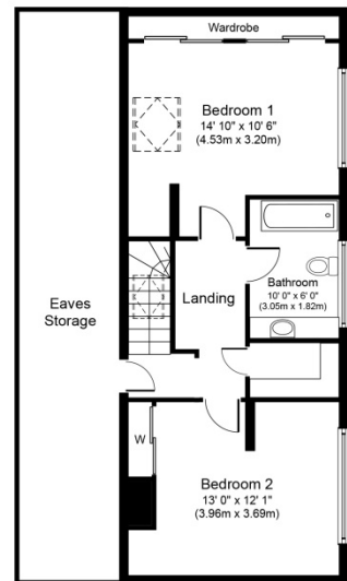
First Floor Approximate Floor Area 581 sq. ft. (54.0 sq. m.)
